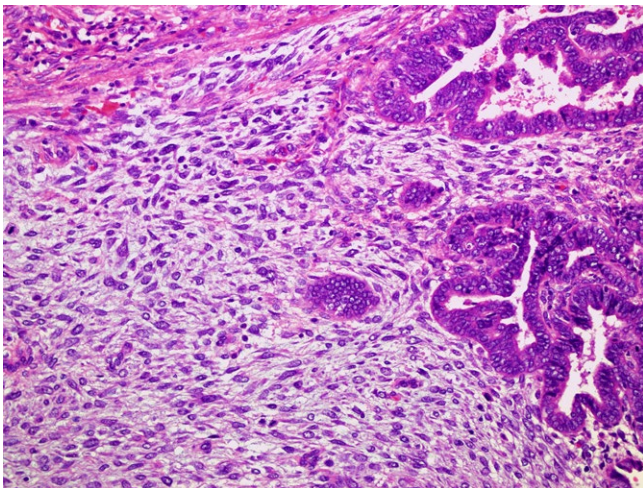
FIGURE 4 Carcinosarcoma.
