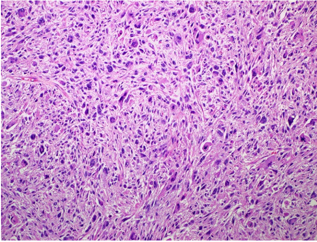
FIGURE 1 Leiomyosarcoma.
