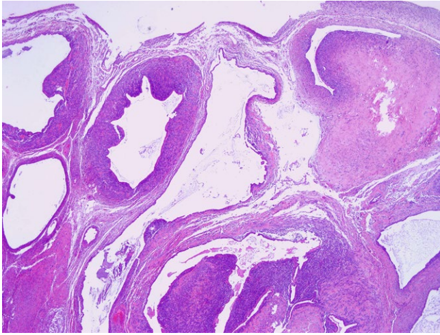
FIGURE 3 Adenosarcoma.
